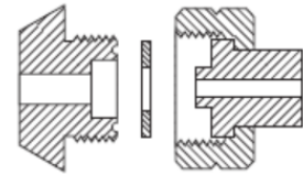
CGA 670 1.030-14NGO-LH-EXT (Face Washer)
