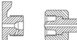
CGA 326 .825-14NGO-RH-EXT (Small Round Nipple)
