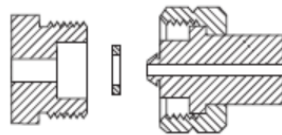
CGA 678 1.030-14NGO-LH-EXT (Recessed Washer)
