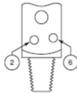
CGA 880 Pin-Indexed Yoke, Pins 2-6
