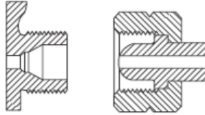
CGA 555 .903-14NGO-LH-EXT
