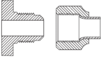
CGA 440 .875-14UNF-2A-RH-EXT (5/8" SAE Flare)
