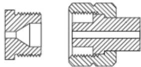
CGA 677 1.030-14NGO-LH-EXT (Round Nipple)
