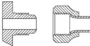
CGA 295 .750-16UNF-2A-RH-EXT (1/2" SAE Flare)
