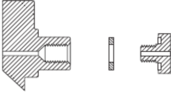
CGA 110 .3125-32UNEF-2B-RH-INT
