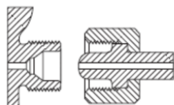
CGA 346 .825-14NGO-RH-EXT (Large Round Nipple)
